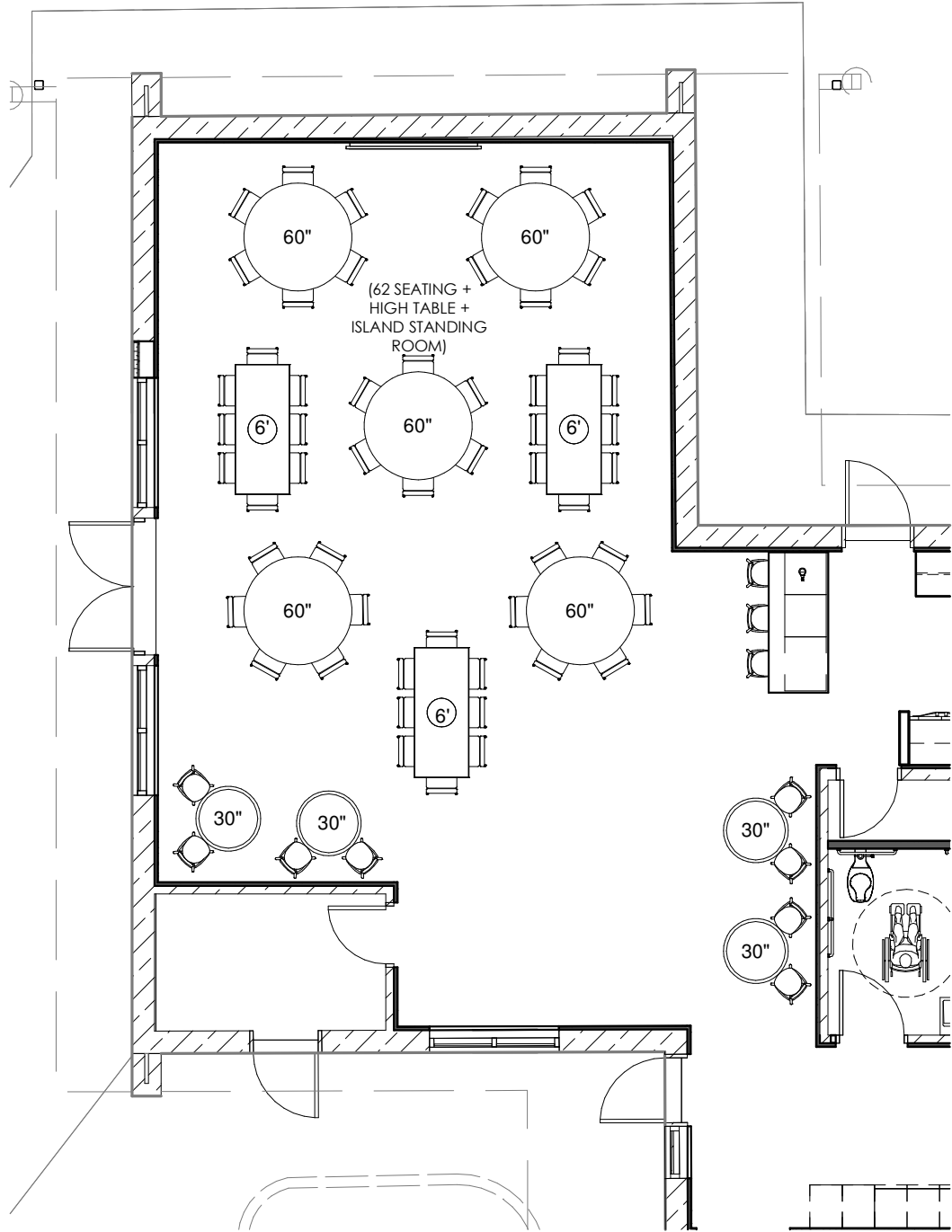
1 PLAN- Social Setup L3 1/8" = 1'-0"
